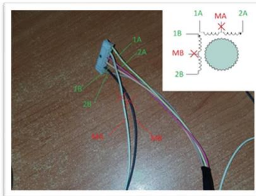
Fig. 13. Stepping motors
