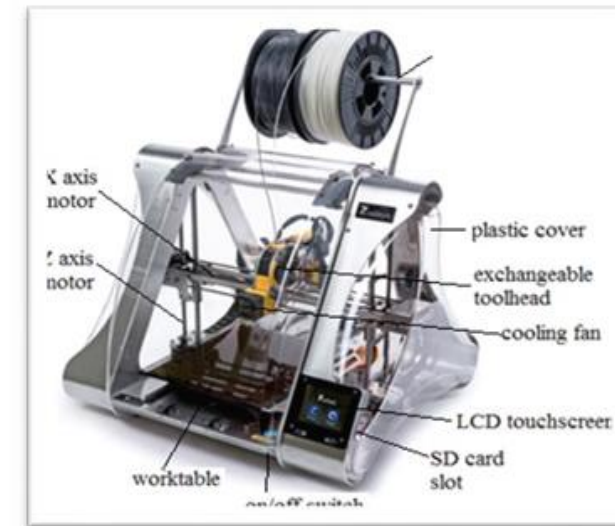
Fig.6. Commercial 3D hybrid printer ZMorph [7]
