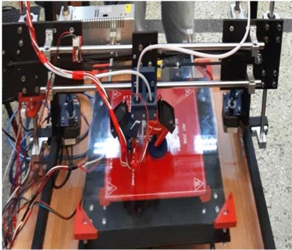
Fig.23. FDM extruder on the 3D hybrid printer
