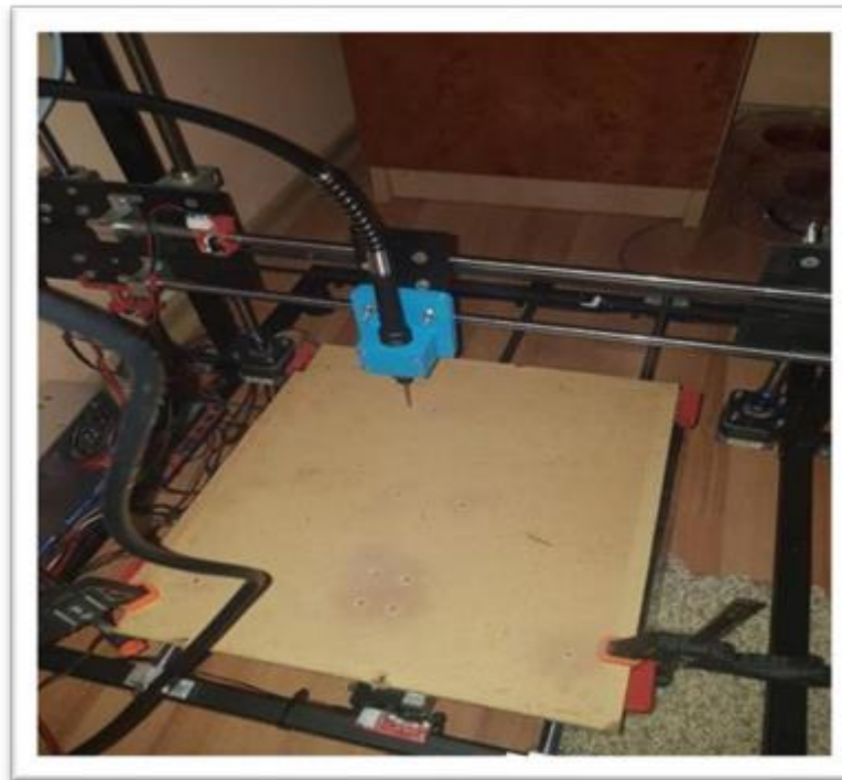
Fig.22. CNC drilling on the 3D hybrid printer
