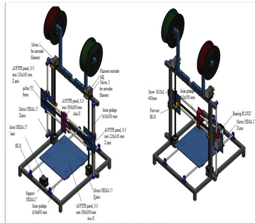
Fig.20. Components of hybrid 3D printer
