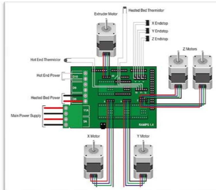
Fig.10. Electrical installation scheme
